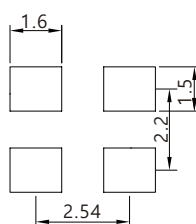
Land Pattern
