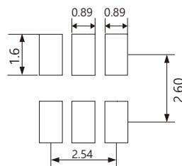
Land Pattern
